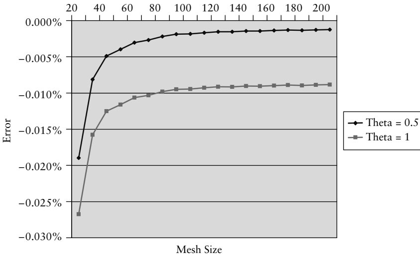
FIGURE 4.1 ADI scheme: convergence for dx, dy \rightarrow 0 .
