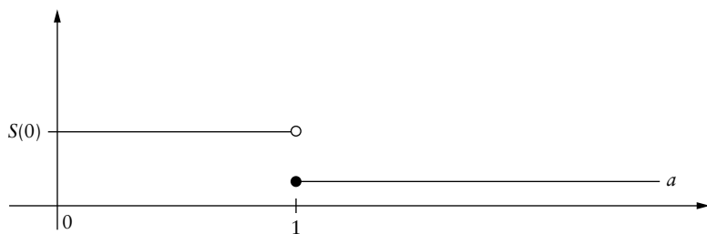
FIGURE 2.1 \omega = a .
