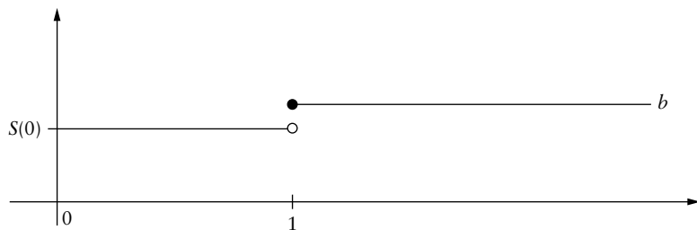
FIGURE 2.2 \omega = b .
