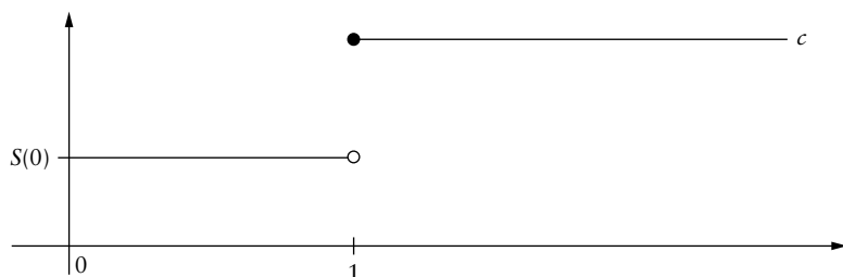
FIGURE 2.3 \omega = c .
